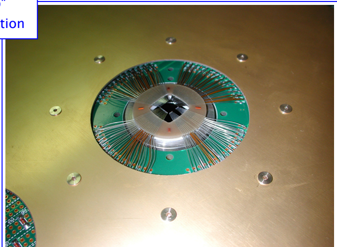
150 °C high temperature probe card with HeatShield and Air Cooling Device
